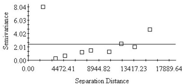
Isotropic Variogram (Covariate- Temp)
